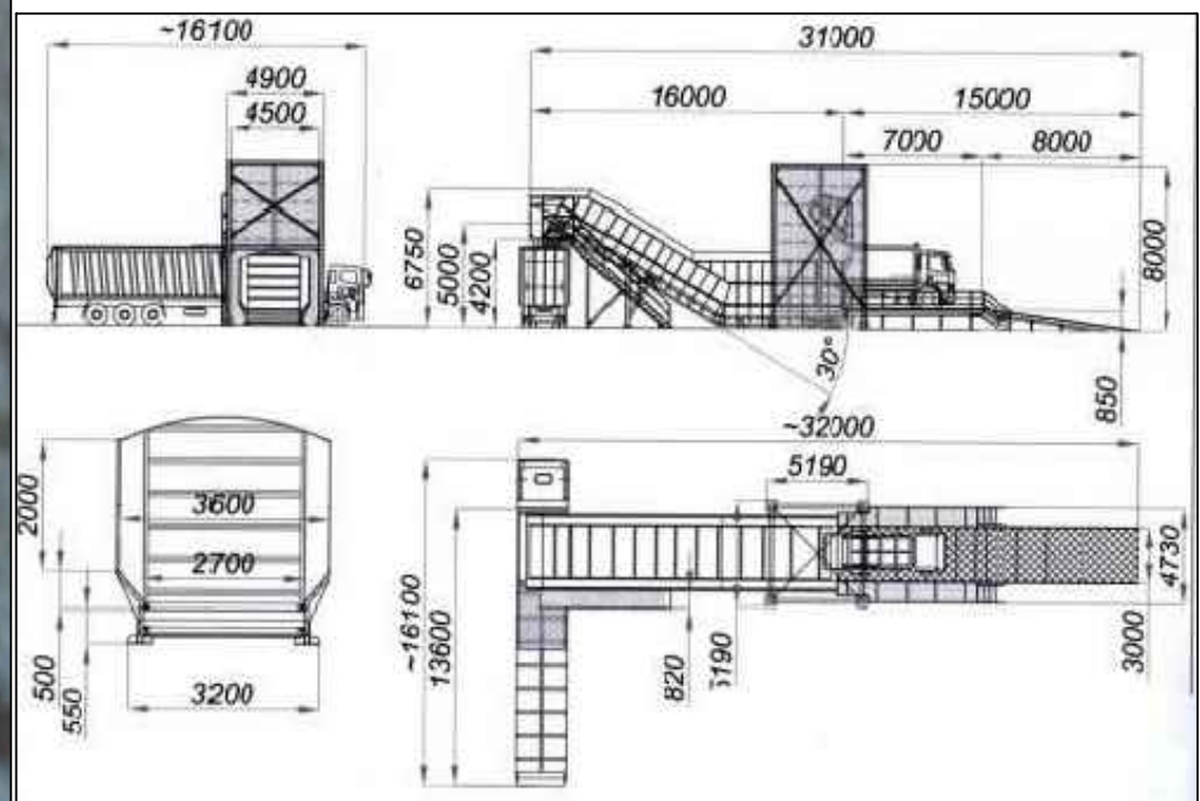
DETAILS OF WASTE TRANSFER SYSTEM
